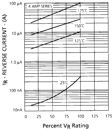
FIGURE 4 Typical Reverse Current vs Applied Reverse Voltage
